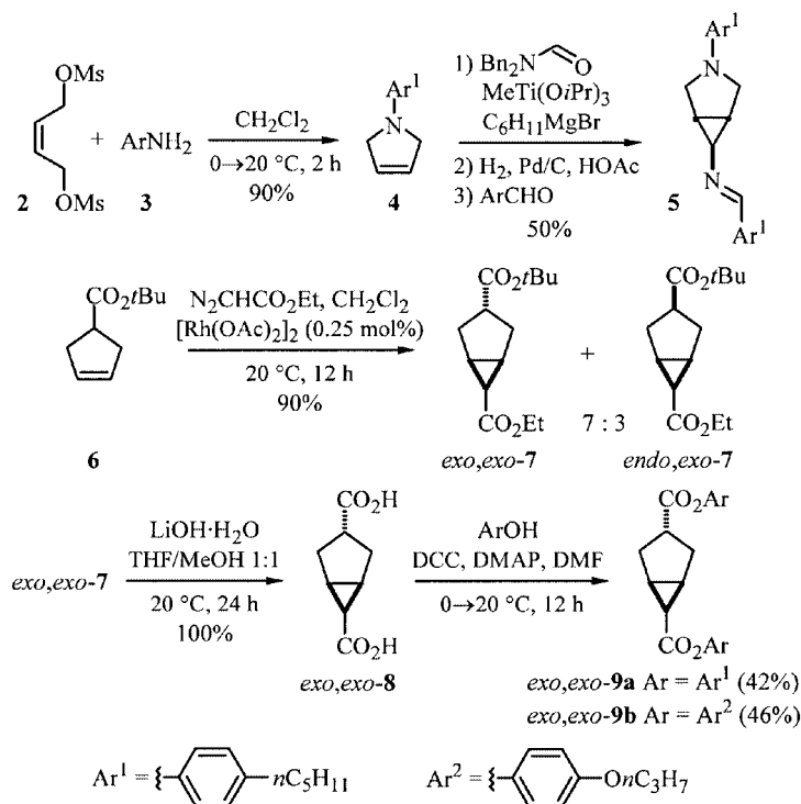
Scheme 1. Syntheses of 3-aryl-6- exo -(arylmethyleneamino)-3-azabicyclo[3.1.0]hexane 5 and diaryl bicyclo[3.1.0]hexane-3,6-dicarboxylates 9a,b
