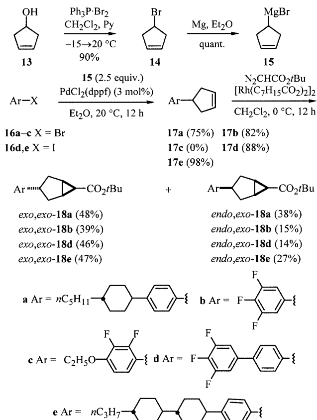
Scheme 2. Preparation of 4-arylcyclopentenones 17 and their dirhodium tetraoctanoate catalyzed cyclopropanation with tert -butyl diazoacetate
